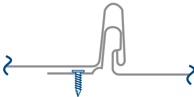
Typical Panel Lap Detail
